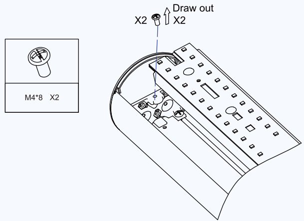
Step 2 : Unscrew the screws and remove the reflector
