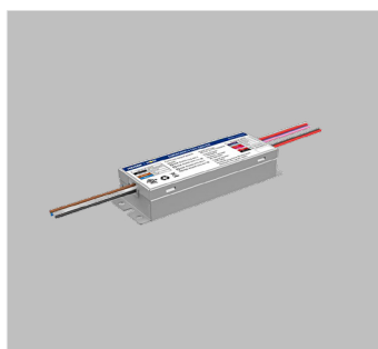
Internal Mount | Lithium | 8W | 100-347Vac | 7.2V 2600mAh | 50/60Hz | Emergency duration: ≥90mins R83006
