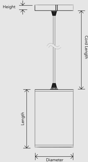
Cord Mount
