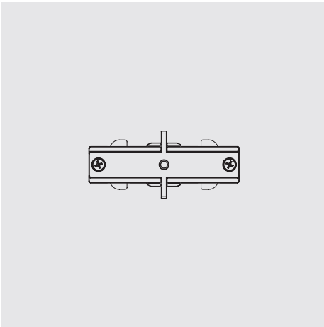
"I" Connector W 79.5 mm (3.13") x H 35.5 mm (1.38")
