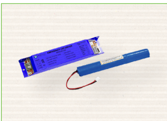
R83004 RENO-EM-C08 Emergency LED Driver (100-347V AC, 50-60Hz, 8W)
